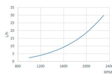
Consumo combustible
